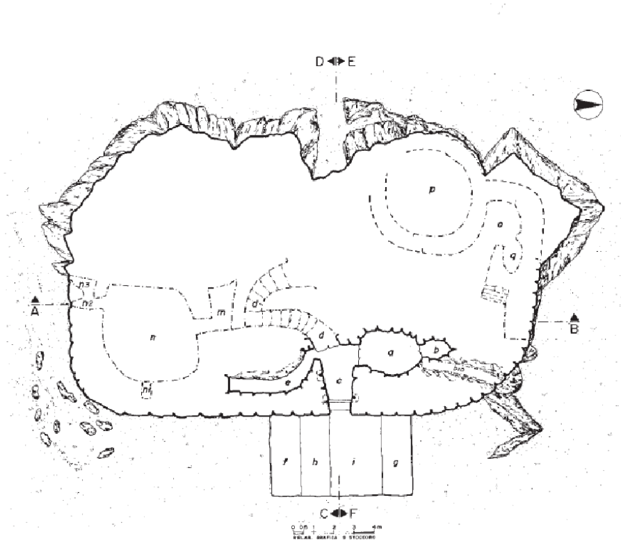
Fig. 1 - Nuraghe Albucciu, ground floor plan (from ANTONA RUJU, FERRARESE CERUTI 1992, fig. 12).
