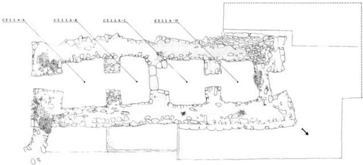
Fig. 1 - Megaron 1 temple plans (from FADDA 2012, fig. 9 page 10).
